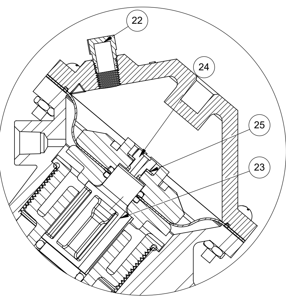
1070172 (K524-X230-14000) NORMALLY CLOSED
