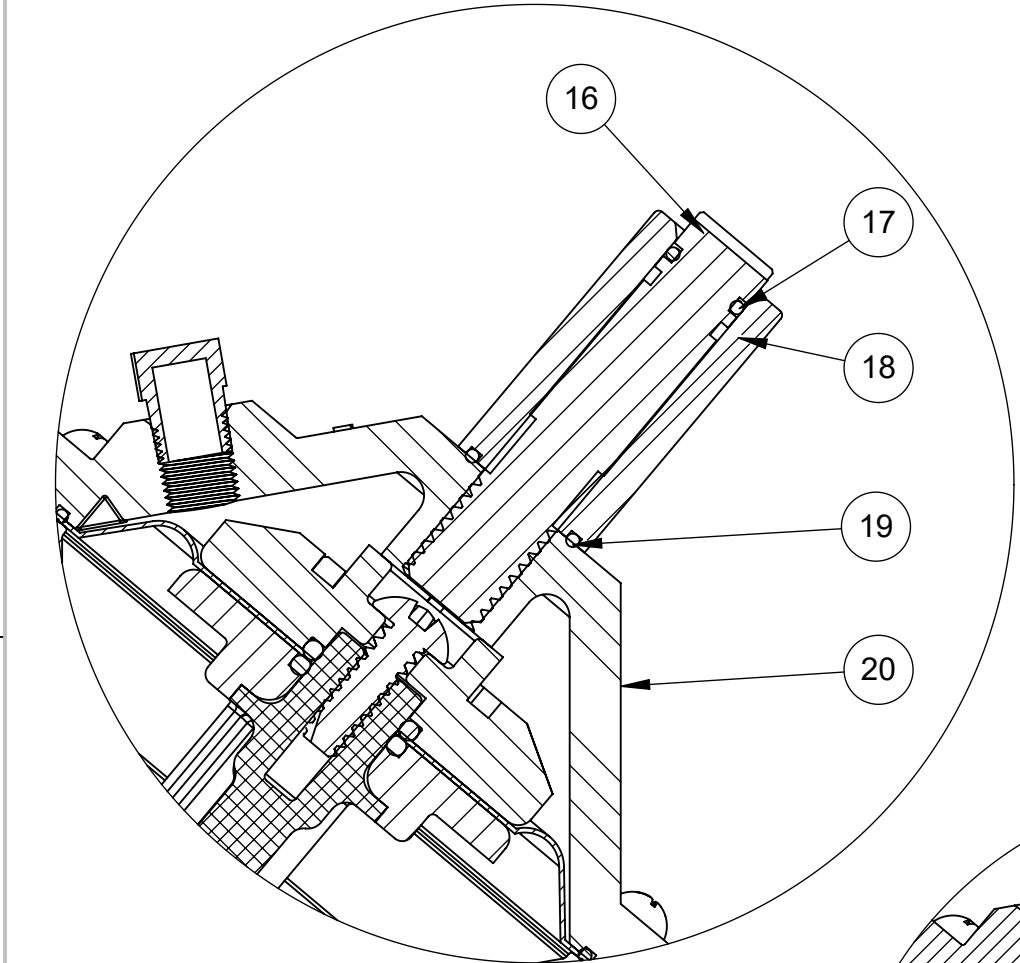
1070170 (K524-X210-14000) LIMIT STOP
