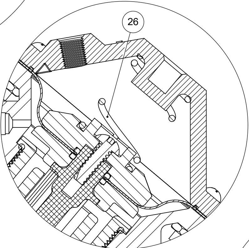
1070171 (K524-X202-14000) SPRING ASSIST CLOSED
